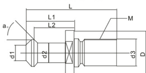
FOR MAS 403
