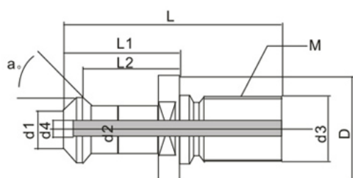
FOR MAS 403
